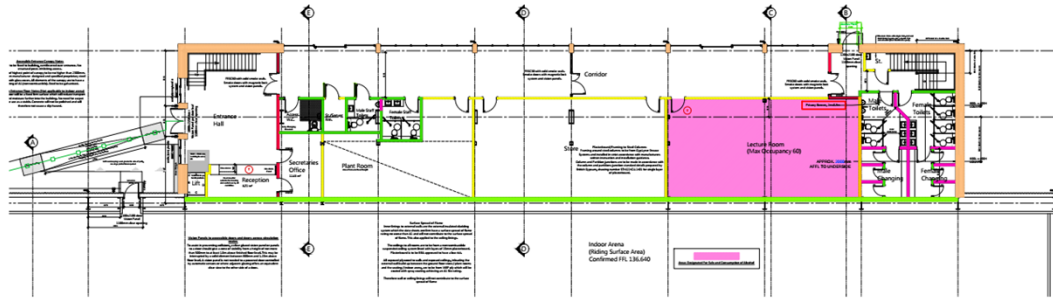
GROUND FLOOR PLAN @ 1:100
